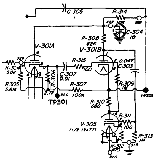
Figure 59. Input Cathode Follower Circuit Diagram. (Components enclosed by broken lines not on etched board.)
