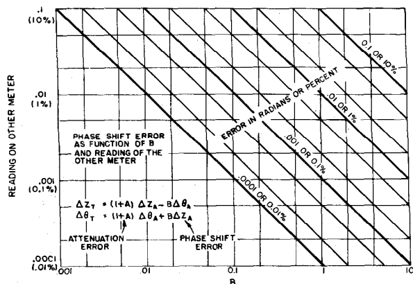
Figure 19. Phase Angle Error as a Function of B and \Delta Z Range.
