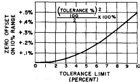
Figure 21. Zero Offset for Correct Reading at Tolerance Limit.
