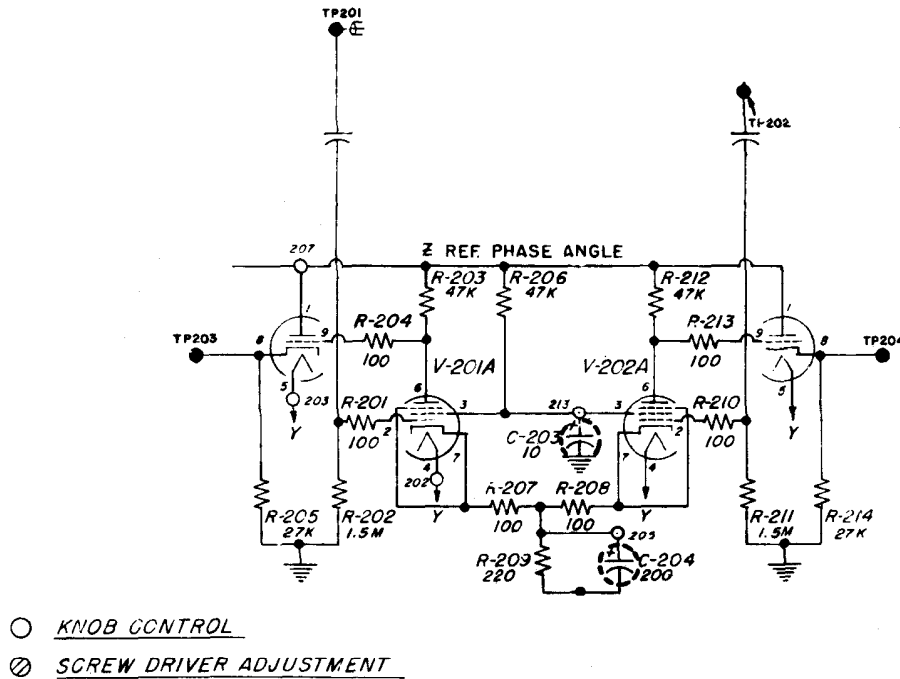
Figure 56. Reference Amplifier Circuit Diagram. (Components enclosed by broken lines not on etched board.)
