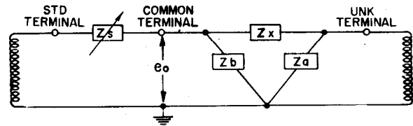
Figure 29. Direct Impedance Measurement Using Variable Standard.
