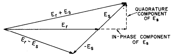
Figure 13. Vector Diagram Illustrating Operation of the Phase-Sensitive Detectors.
