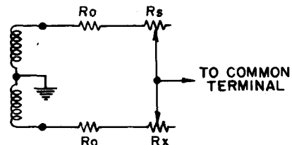
Figure 37. Preferred Setup for Comparison of Rheostats.
