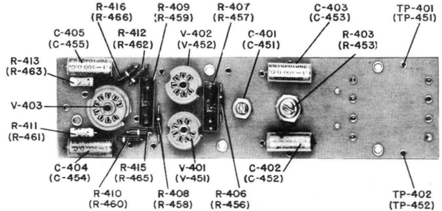
Figure 63. Top View, Detector Circuit Board.
